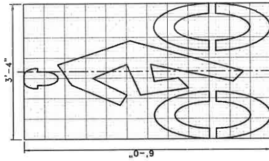
GRID IS 1" SQUARE BIKE LANE SYMBOL
