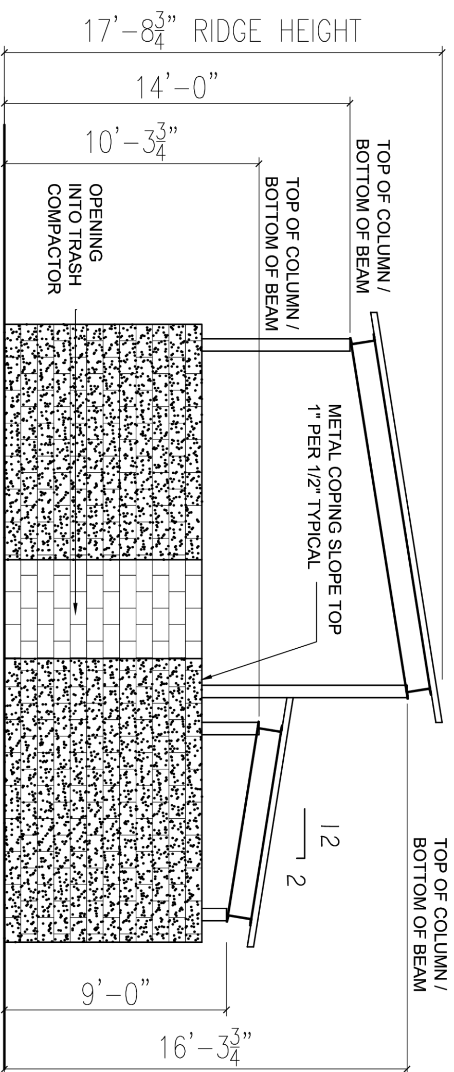
3 BACK ELEVATION
