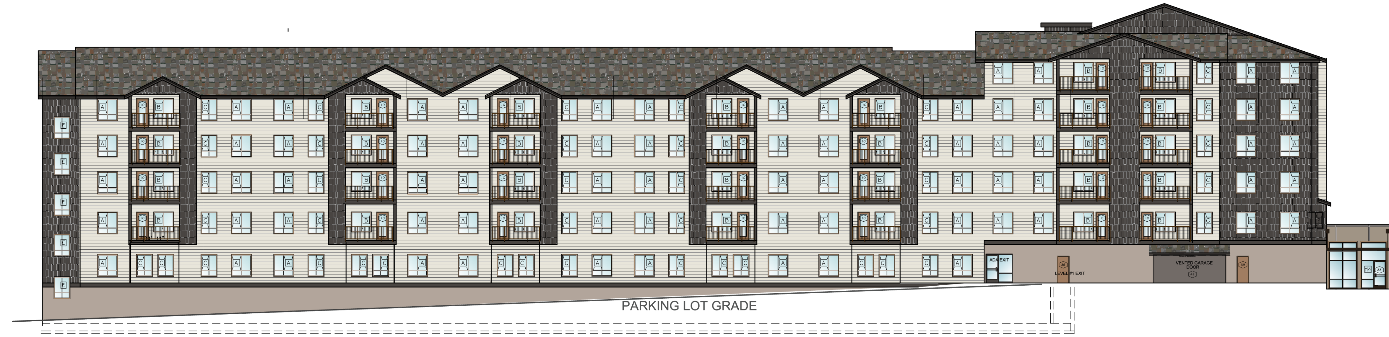
1 SOUTH ELEVATION - BLDG "C"
