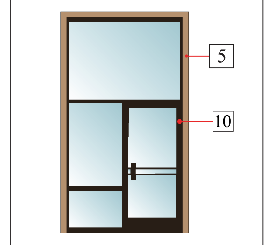
TYP: DOOR & WINDOW: Rec & Commercial Areas - Main Floor
