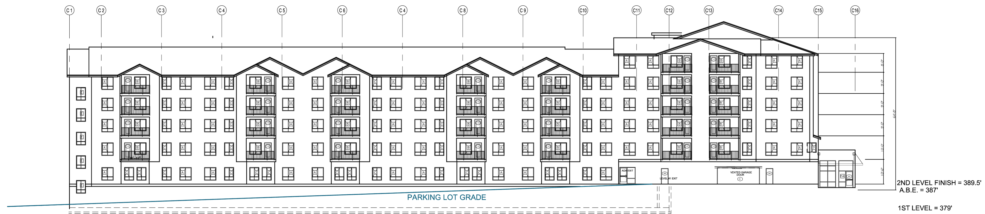
1 SOUTH ELEVATION - BLDG "C"
