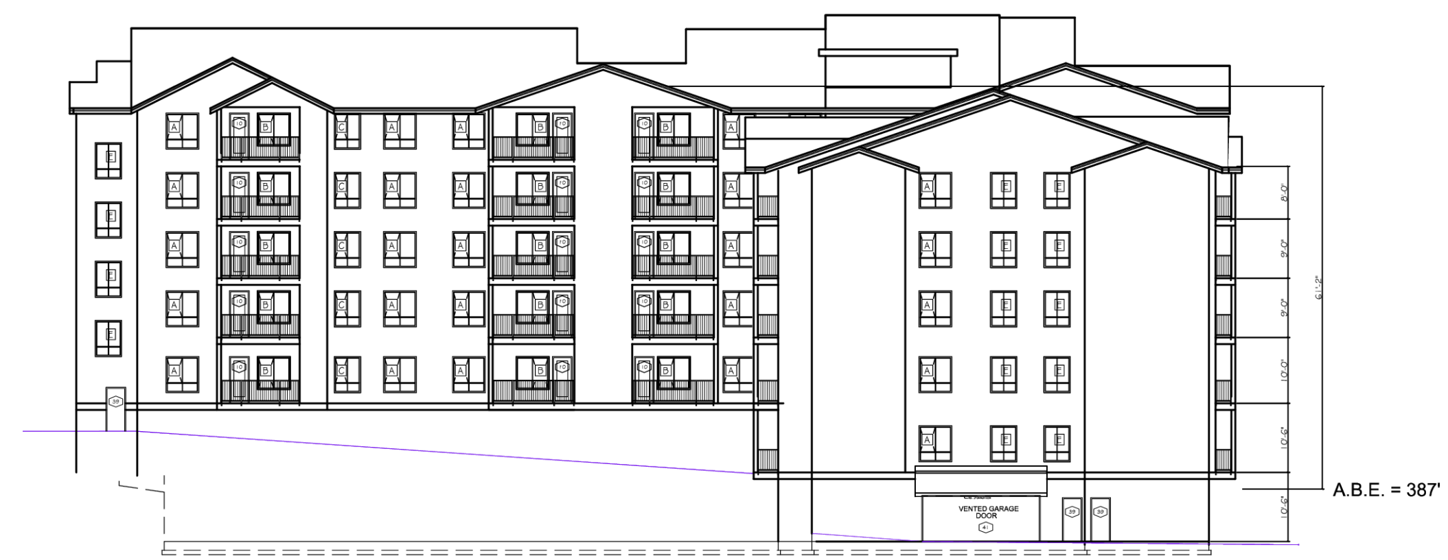
4 WEST ELEVATION - BLDG "C"
